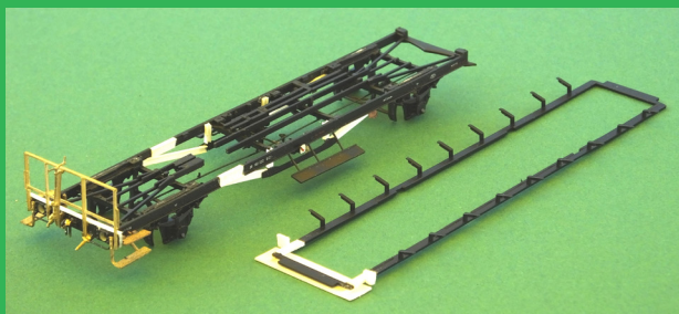
Umbaudetails Band I
